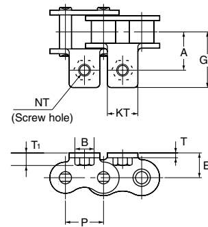
TYPE PA-1
