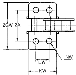
TYPE WK-1
