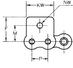
TYPE WSA-1
