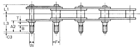
EXTEND PIN WITH SPRING CLIP
