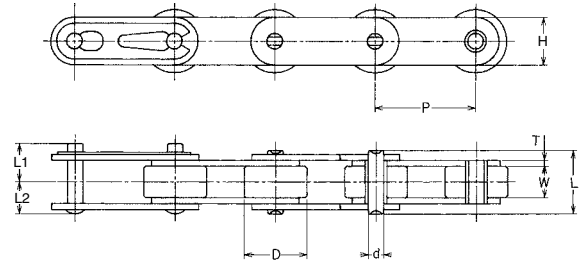
LARGE ROLLER
